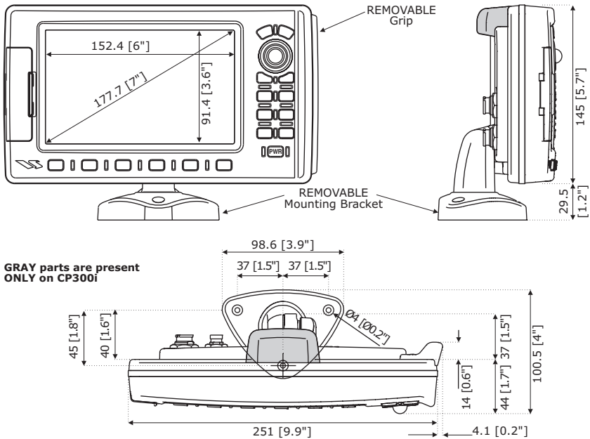
Figure 18.1 - CP300/CP300i Dimensions [mm/inch]
