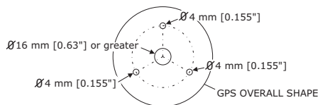
Figure 2.3.0a - Installing the GPS WAAS Smart Antenna (II)
