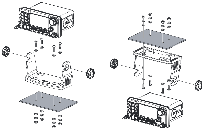
DESKTOP MOUNTING
