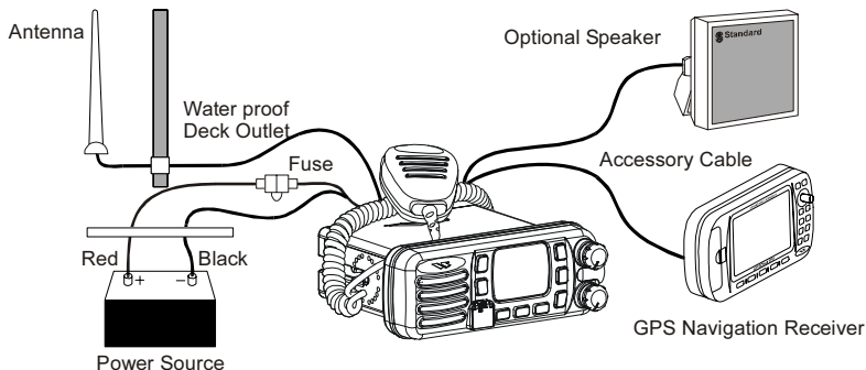
Figure 1. General Installation
