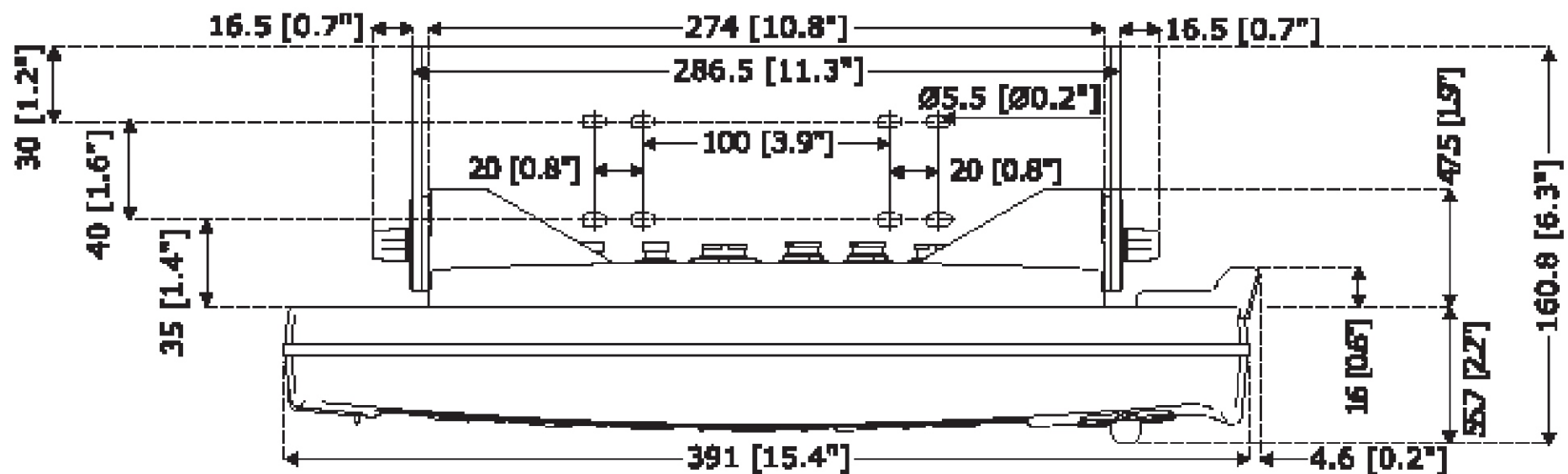
Figure 18.2 - CP500 Dimensions [mm/inch]
