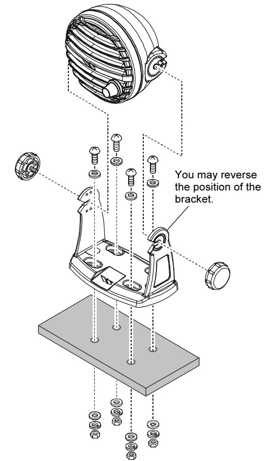
Figure 1 (Desktop Mount)
